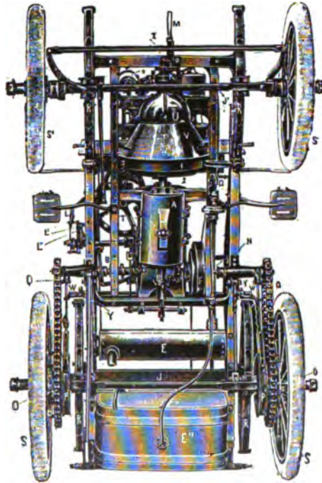
FIG. 373.—Plan of the body and underframe of the average weight Panhard-Levassor Carriage, showing machinery and general apparatus in position. A is the case containing the change speed gear; B, the reversing connections; C, the carburetter; D, the circulation pump; E, the muffler; E', the water reservoir; F, the differential gear case; L, the braking lever; L', the reversing lever; L'', speed changing lever; O, the sprocket on the rear wheels; Q, the driving chain; S, the rear wheels; S', the forward wheels; T, the steering gear; U, the motor case; V, the case enclosing the flywheel and main clutch; W, the attachment for controlling the brakes; X, the adjustable distance rod between the carriage body and the rear wheels; P and P, drums for the band brake; (1), female cone of the main clutch; (2), male cone of the main clutch.
